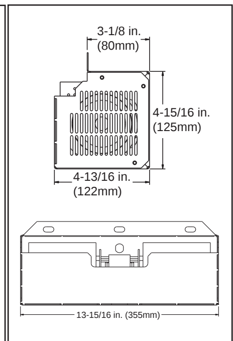
Figure 16.2 - Blower Housing Dimensions
