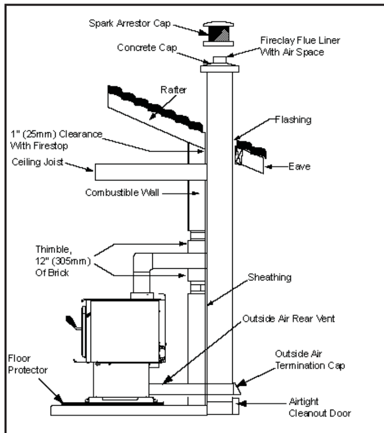
Figure 8.1 Masonry Chimney
