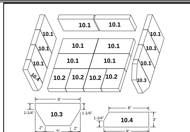
Figure 35.1 - 3100 Millennium Brick Assembly
