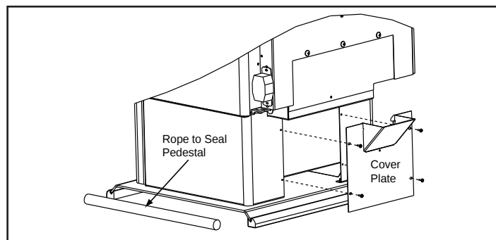
Figure 14.2 - Floor Installation Alternative
