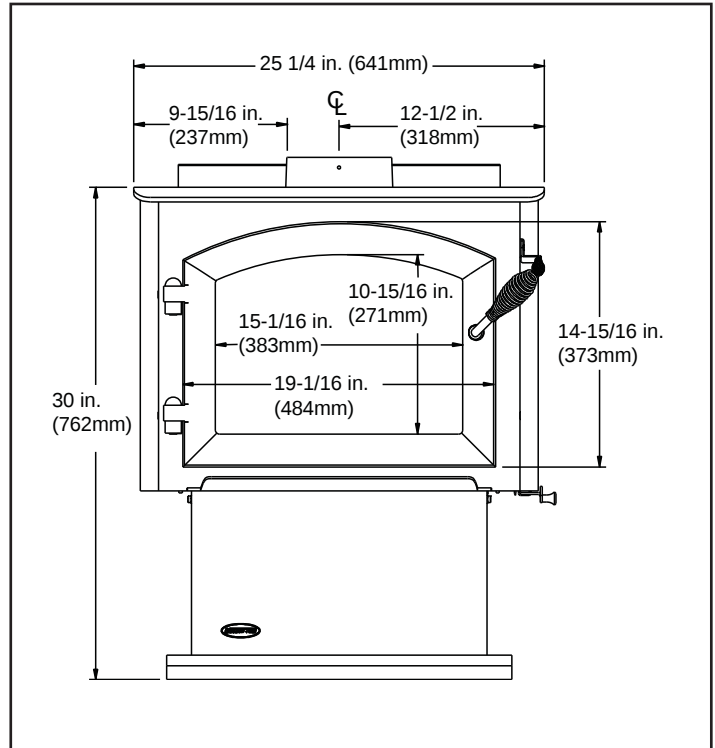
Figure 9.2 Front View
