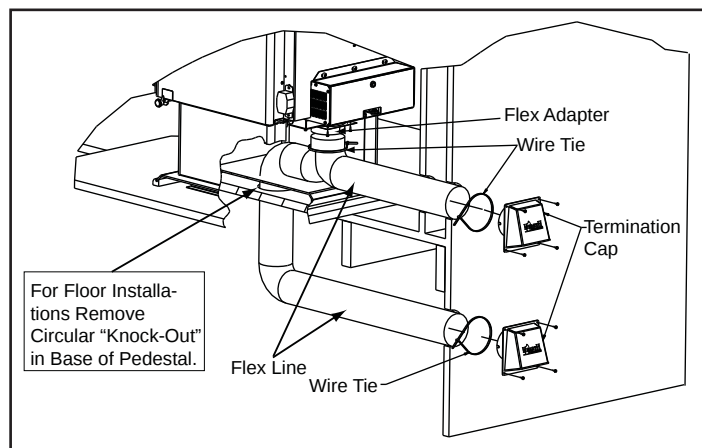
Figure 14.1 - Floor & Rear Installation
