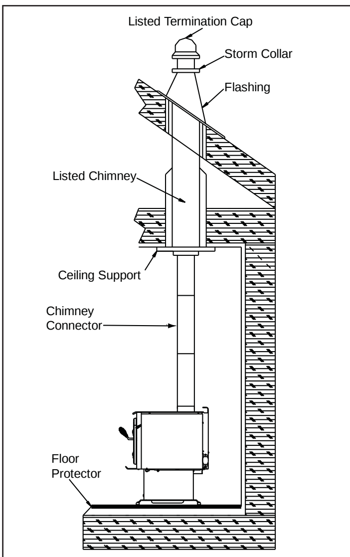
Figure 17.2 - Prefabricated Interior Chimney
