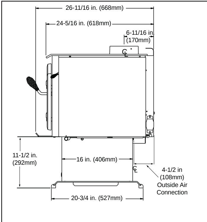
Figure 9.1 Side View
