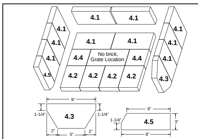
Figure 35.2 - 3100 Step Top Brick Assembly
