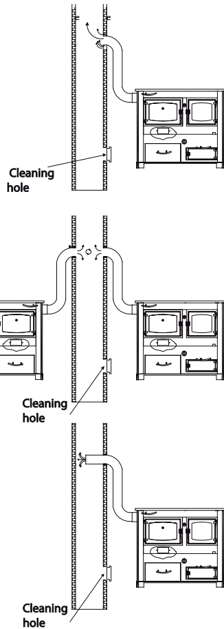
Incorrect cooker connection to chimney
