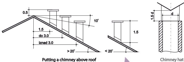
Picture 4. Chimney installation above the roof and chimney cap placement
