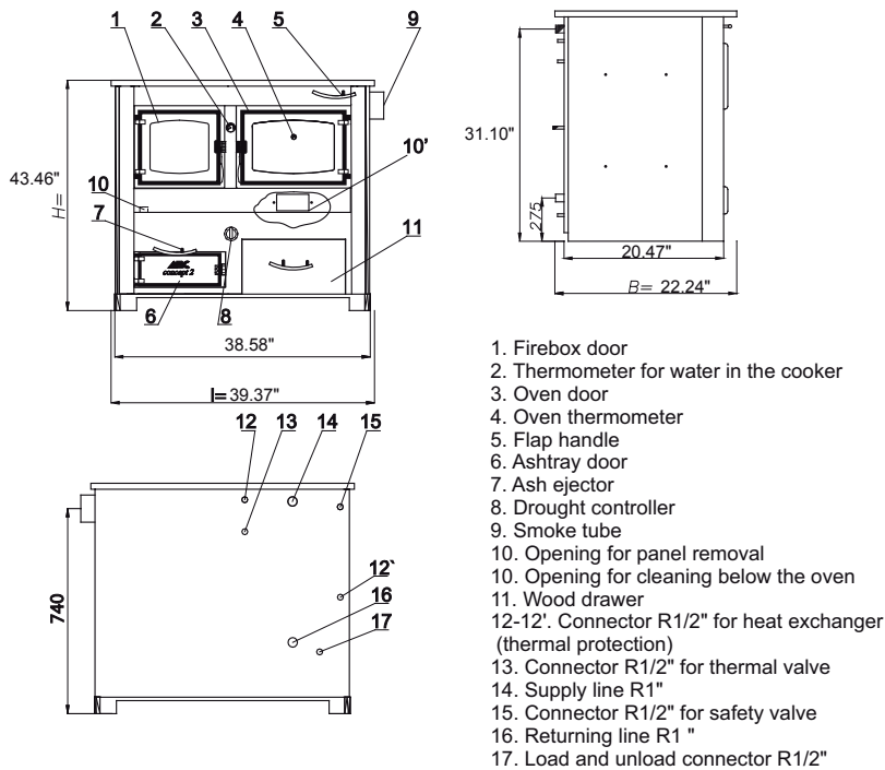
Picture number 1: STOVE FOR CENTRAL HEATING – Concept 2
