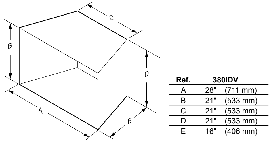
Figure 3 - IDV Fireplace Insert Opening Dimensions
