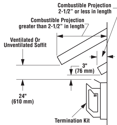
Figure 5—Side Elevation View
