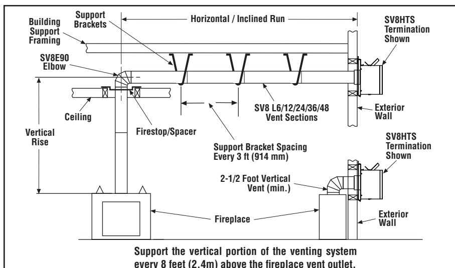
Figure 26—Typical Horizontal Vent Installation
