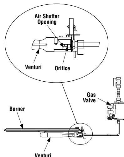
Figure 41 - Air Shutter Adjustment
