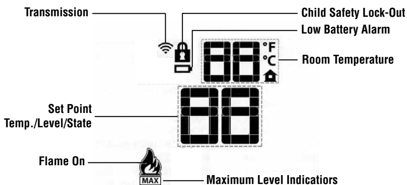
Figure 50 - Indicator Icons
