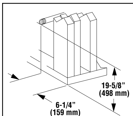
Figure 10 - Right-Front Corner of Fireplace Framing
