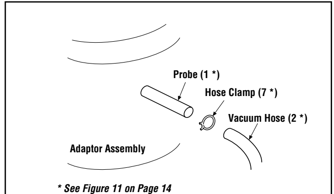
Figure 21 - Vacuum Hose Connection to Probe
