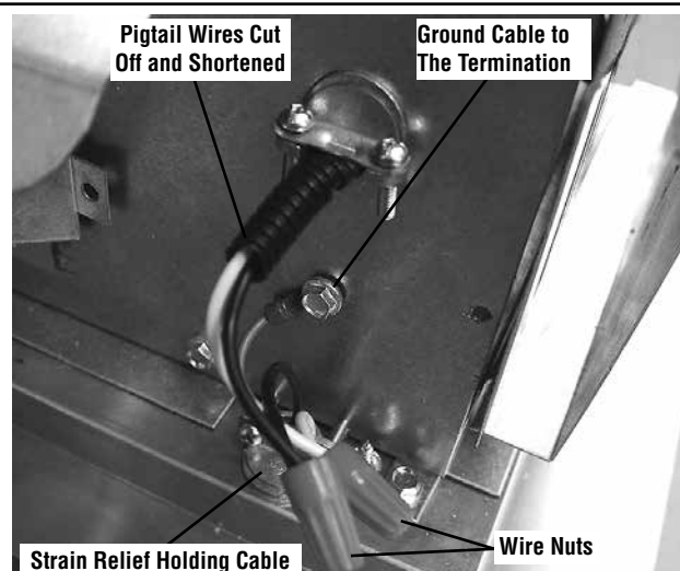
Figure 26 - Junction Box Cover Removed
