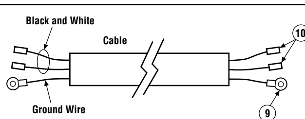
Figure 24 - Cable Connections
