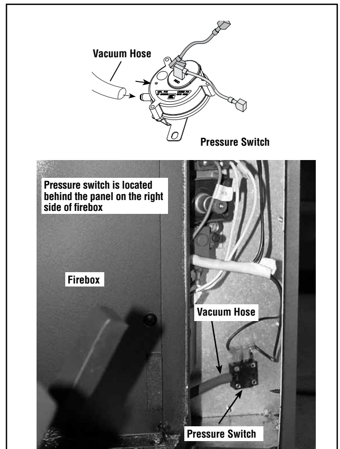
Figure 22 - Vacuum Hose Connection to Pressure Switch
