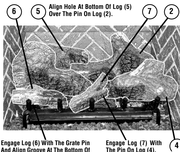
Figure 38 - Placing Logs 5, 6, and 7
