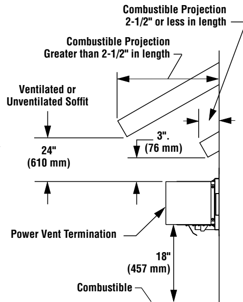
Figure 3 - Horizontal Vent Termination Clearances
