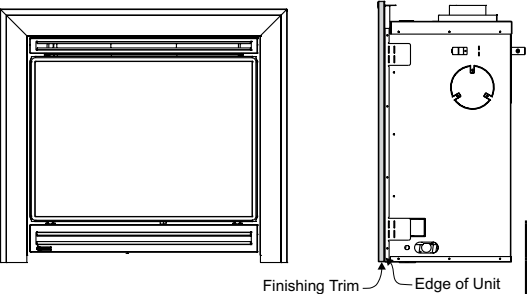
Finishing Trim
