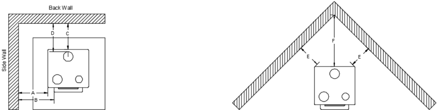
Figure 4. Parallel installation & Corner installation
