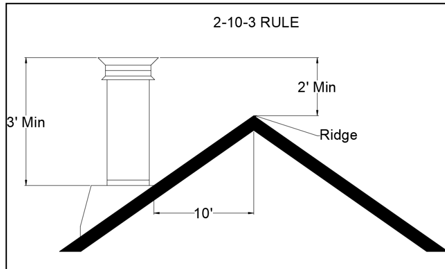
Figure 8. Chimney height requirements
