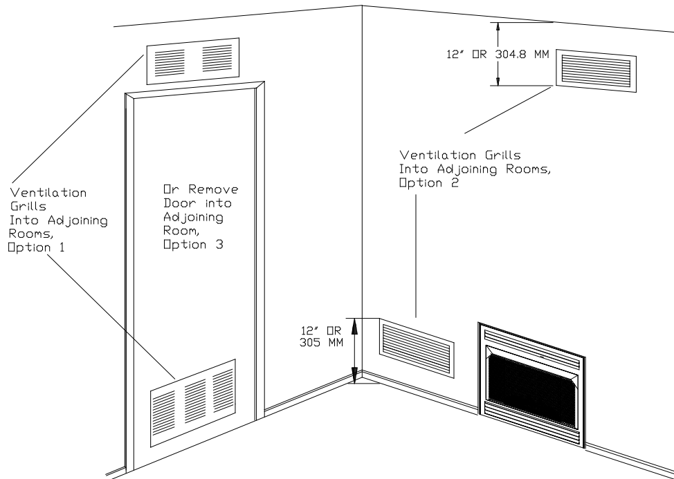
Figure 13 Ventilation Air From Inside Building
