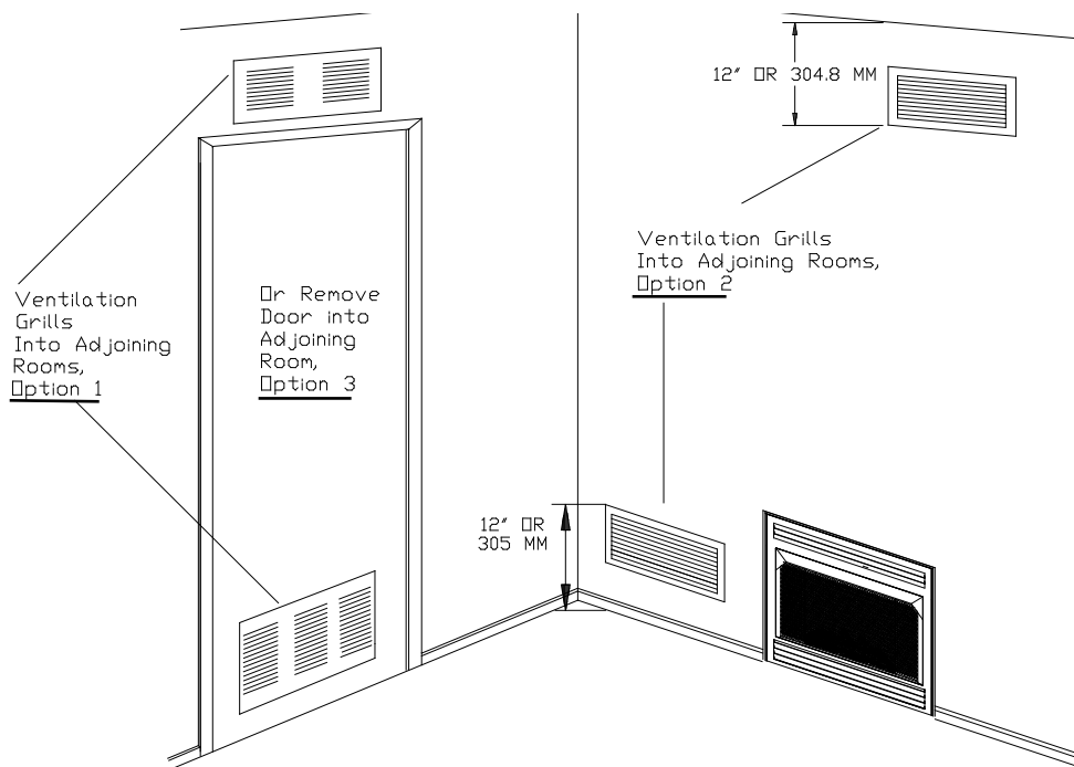
Figure 6 Ventilation Air From Inside Building
