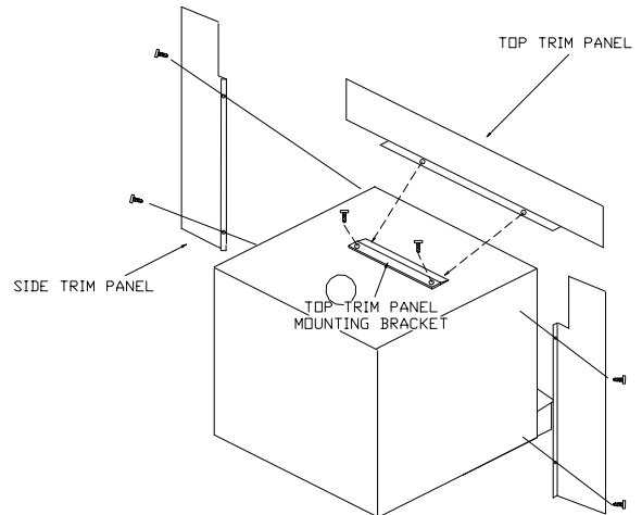
FIGURE 3 MOUNTING TRIM PANELS
