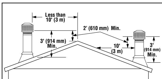
Figure 1 - Chimney Height Requirements
