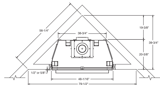
CORNER INSTALLATION
