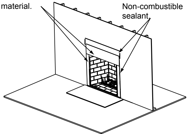
Figure 9.1 Non-combustible Facing
