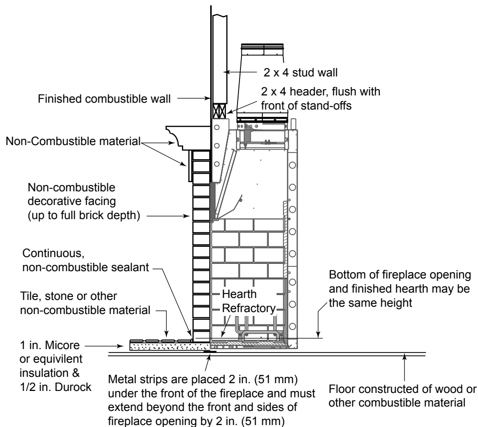
Figure 9.2 Decorative Facing
