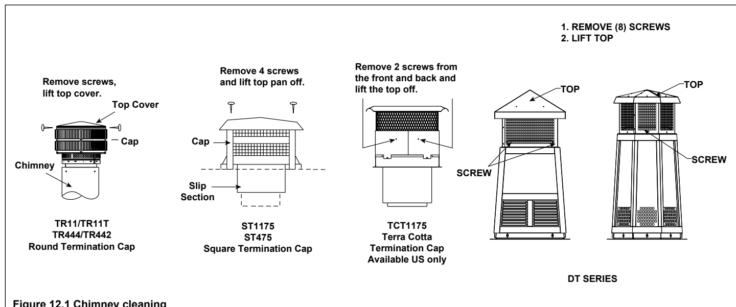
Figure 12.1 Chimney cleaning
