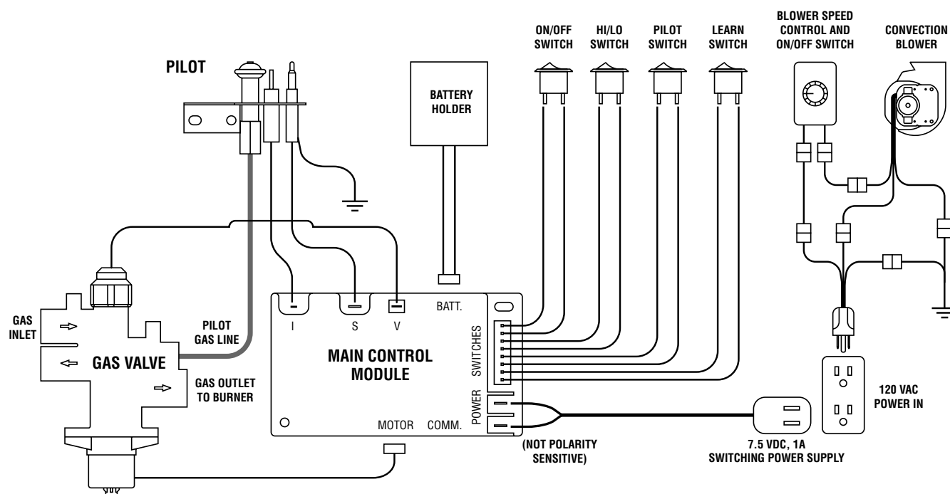
Figure 25 - Electronic Control Schematic - Models Bremerton™ 27 & 32
