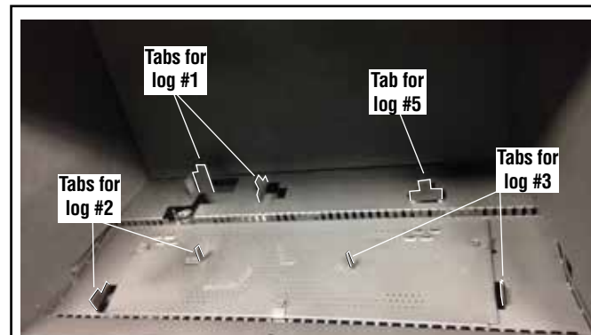
Figure 14B - Locate the log placement tabs, BRMTN32
