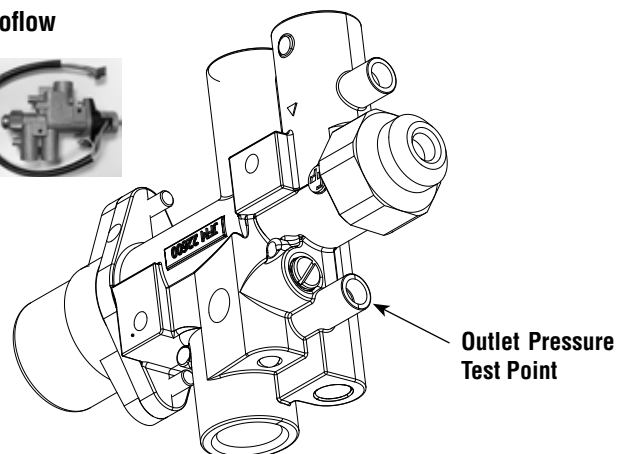
Figure 19A - MANIFOLD Outlet Gas Pressure Test Point
