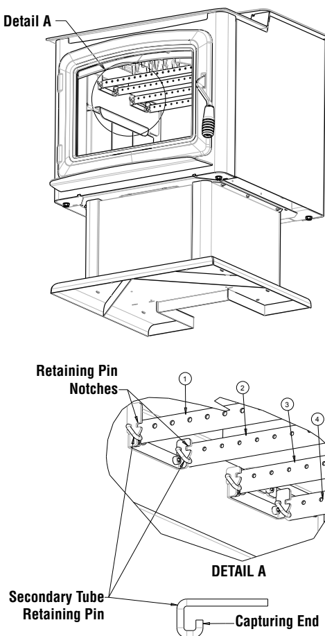
Figure 26 - Secondary Air Tube Retainers
