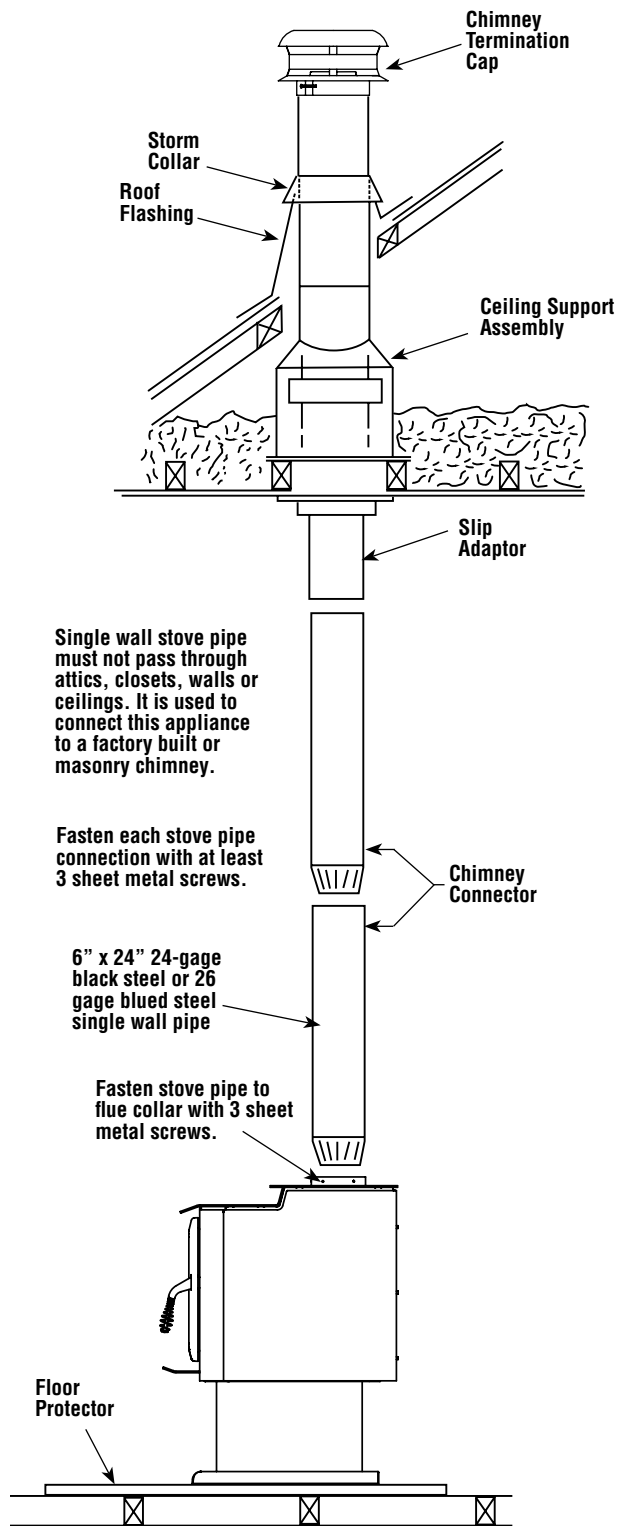
Figure 9 - Typical Installation
