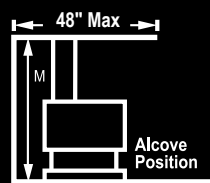
Minimum Clearance to Combustible Materials - Inches
