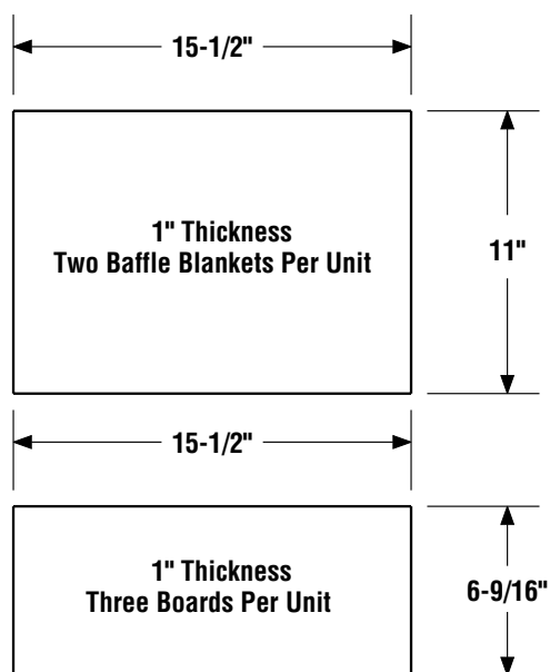
Figure 16b - Baffle Insulation Parts
