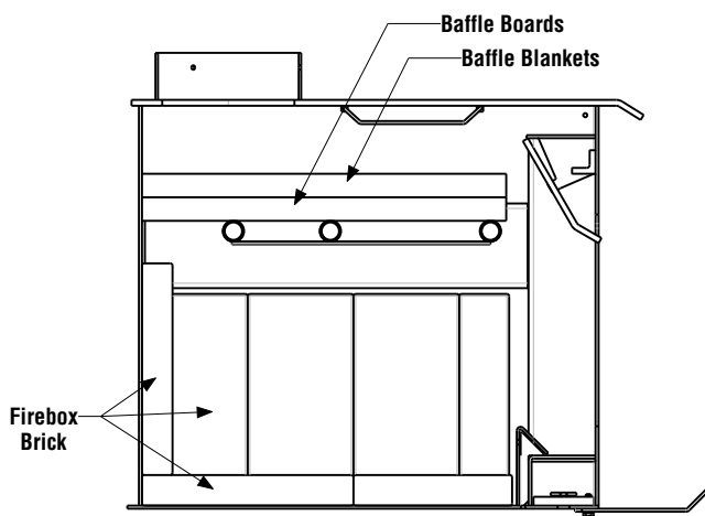
Figure 16a - Side Cut-A-Way View of Firebox
