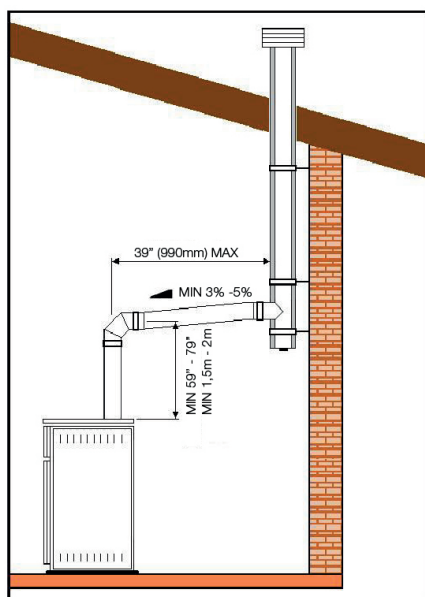
Vertical installation, prefabricated interior chimney
