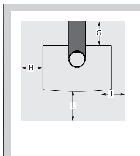
Figure 11: Floor Protection
