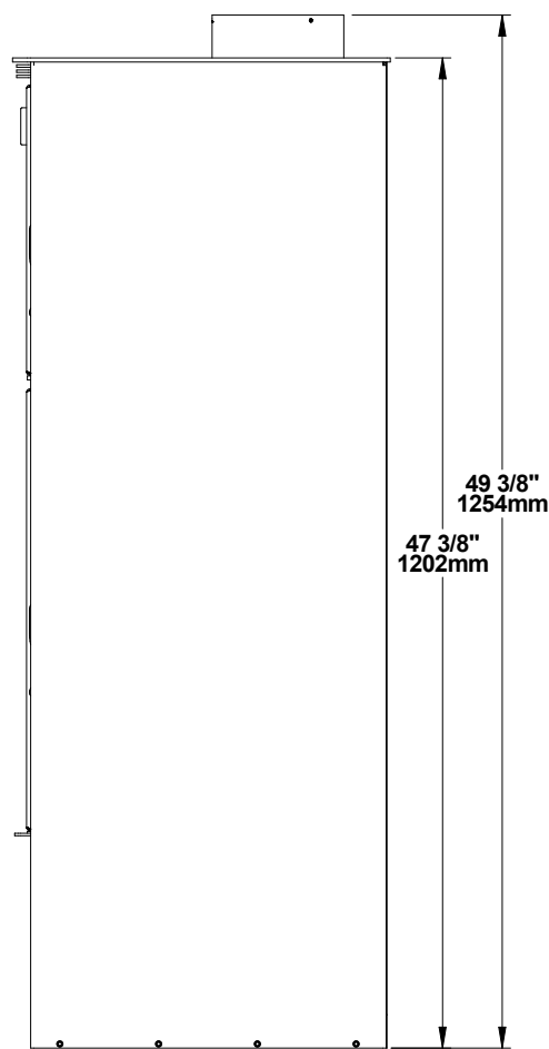
Figure 3: Side view
