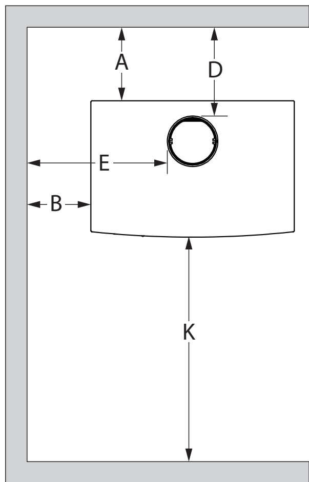
Figure 8: Clearances - Top
