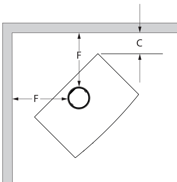
Figure 10: Clearances - Corner
