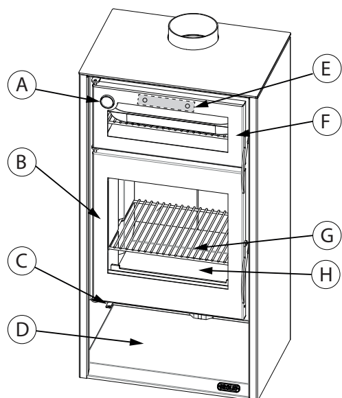
Figure 4: Component Location
