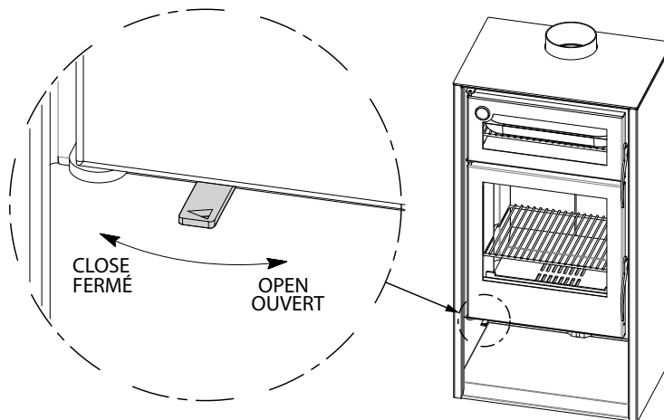
Figure 6: Air inlet control
