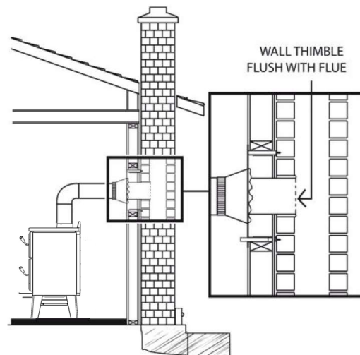
Figure 44: Masonry hearth installation
