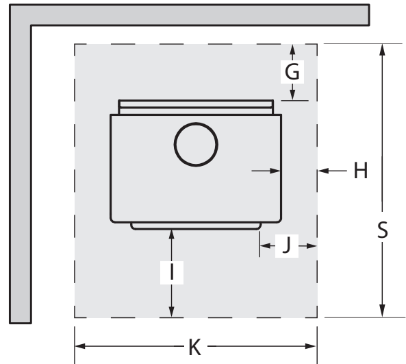
Figure 38: Floor protection
