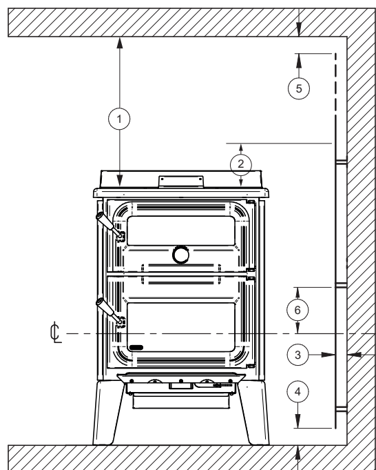
Figure 41: Clearances with Heat Shield - Face
