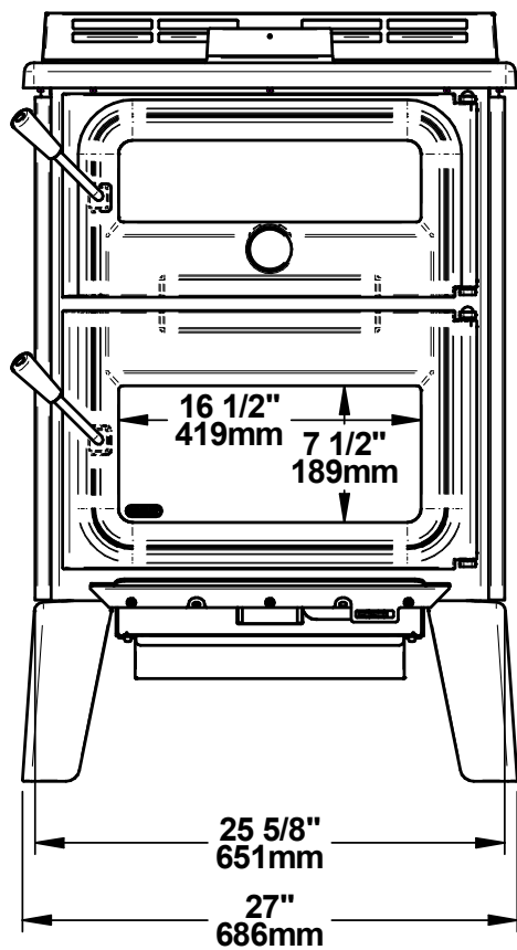
Figure 2: Front view
