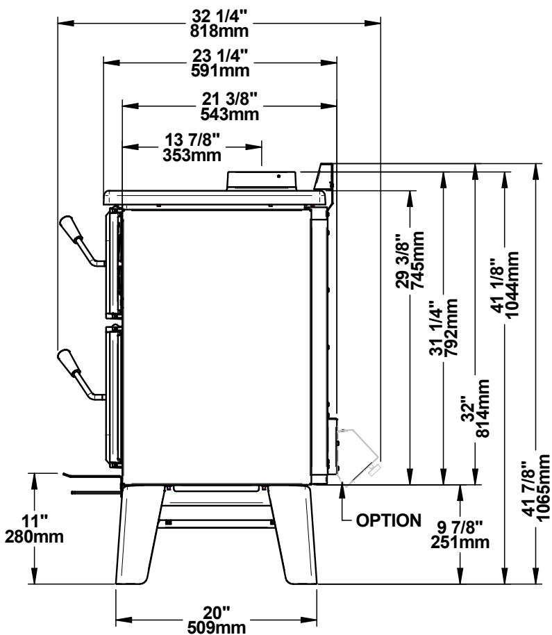
Figure 3: Side view
