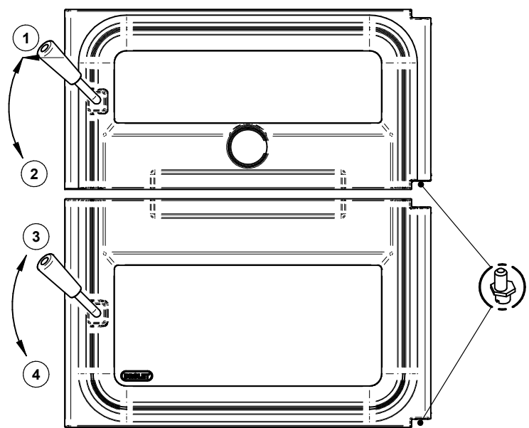
Figure 32: Doors adjustment
