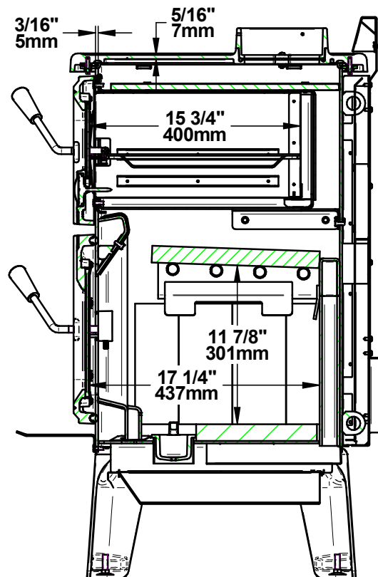
Figure 6: Side view : Combustion chamber
