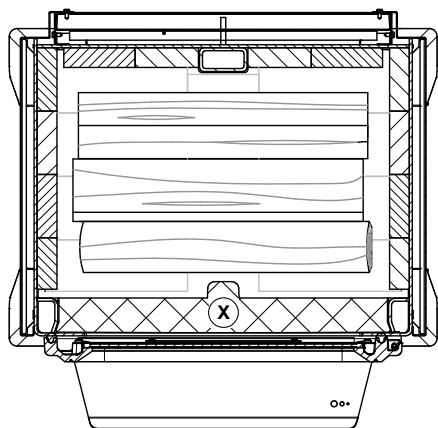
Figure 16: Position of the bottom pieces (Medium burn)
