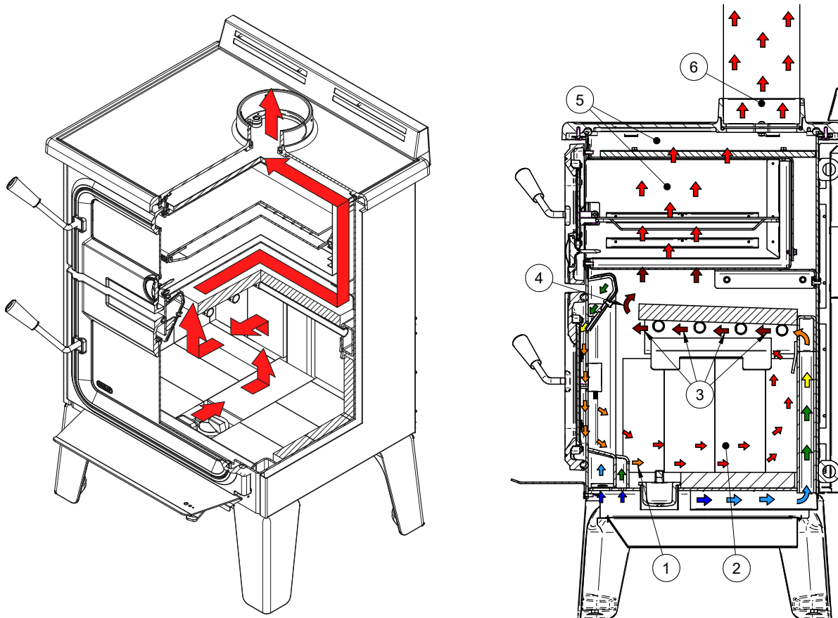
Figure 23: Gas path
