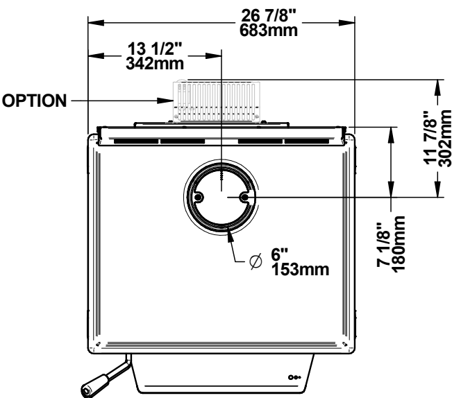
Figure 1: Top view
