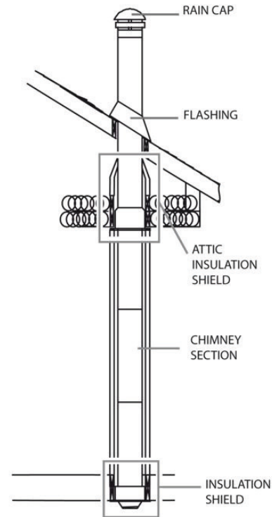
Figure 24: Standard installation
