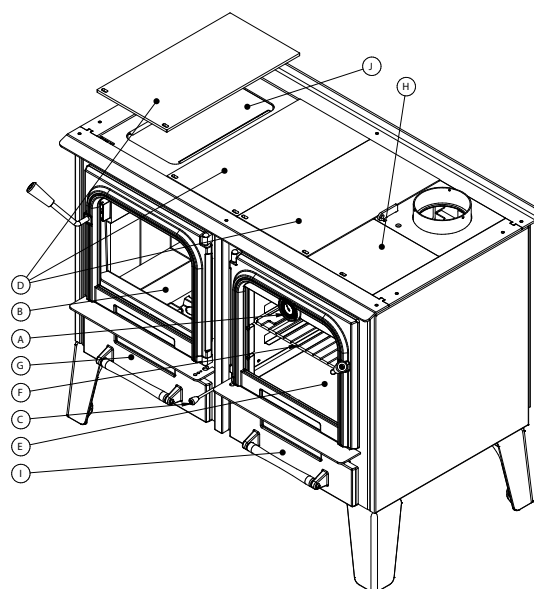
Figure 1: Component Location
