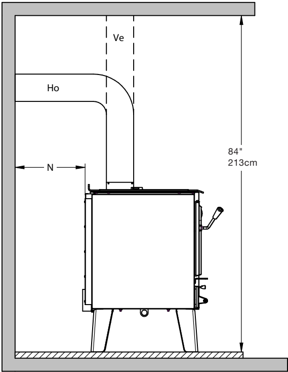
Figure 16: Clearances – Top
