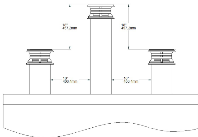
Figure 26: Flat roof
