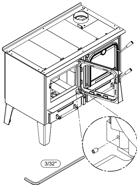
Figure 9: Release eccentric hinges
