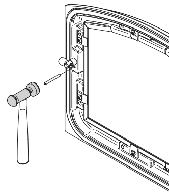
Figure 8: Installing the split pin
