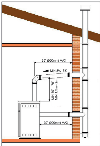
Vertical or horizontal installation, prefabricated exterior chimney
