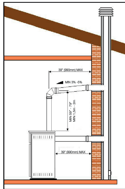
Vertical or horizontal installation, masonry exterior chimney
