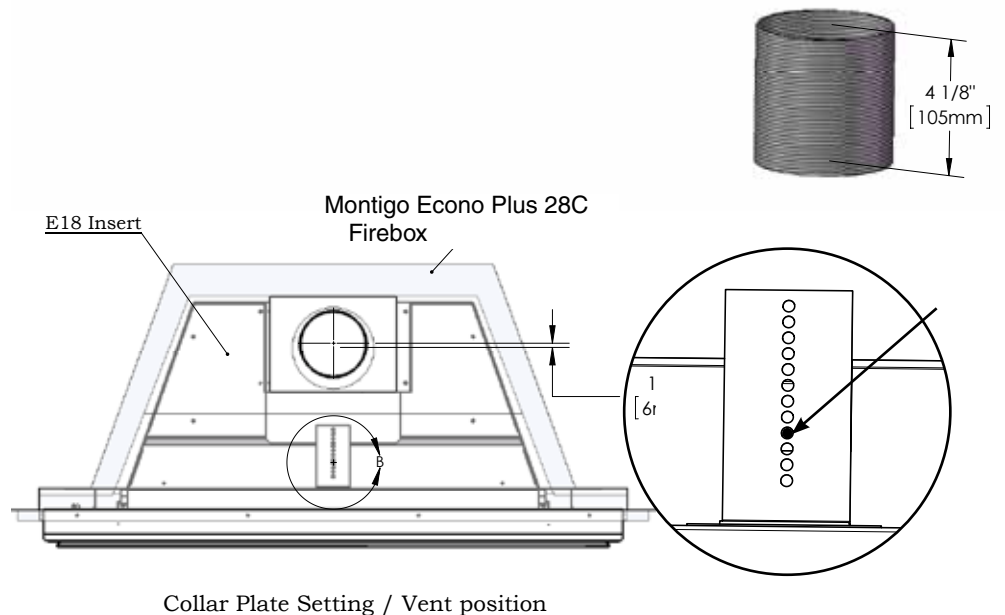
Collar Plate Setting / Vent position
