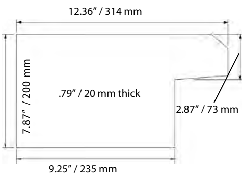
Bottom Side Firebrick (Stanford 140 & Harmony III) order code: 41198
