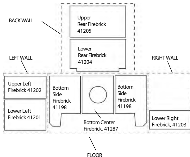
Stanford 140 & Harmony III Firebrick Placement Diagram
