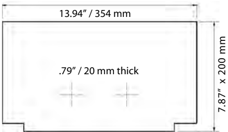
Lower Rear Firebrick (Stanford 140 & Harmony III) order code: 41204
