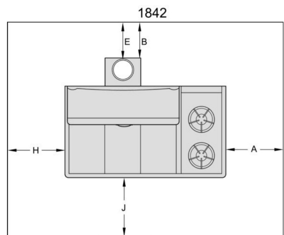
Corner Installation - All Models
