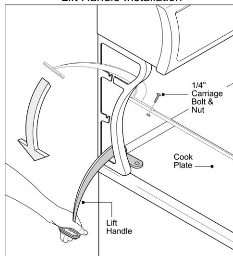
Lift Handle Installation
