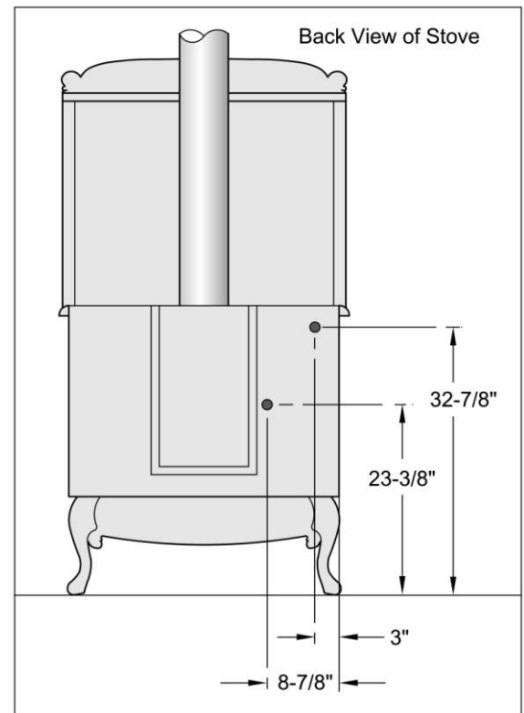
Location of Waterjacket Holes for Rough-in Calculations
