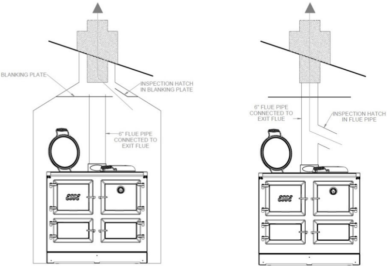
FIGURE 22: LOCATION OF MAIN FLUE INSPECTION HATCH.
