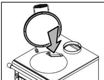
Hotplate removal
