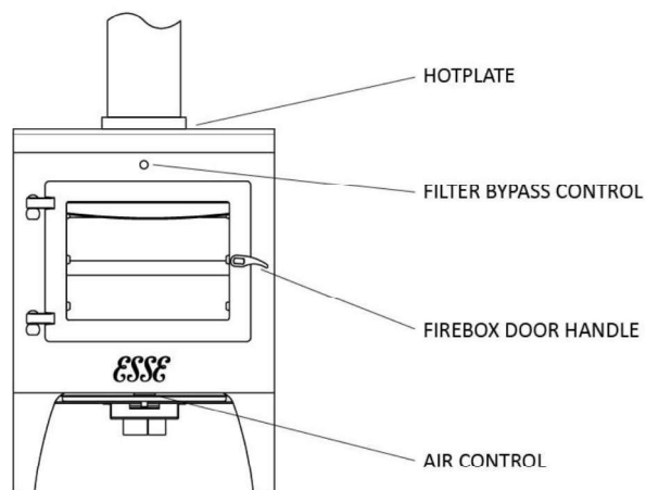
Figure 2 Warmheart S Stove Controls
