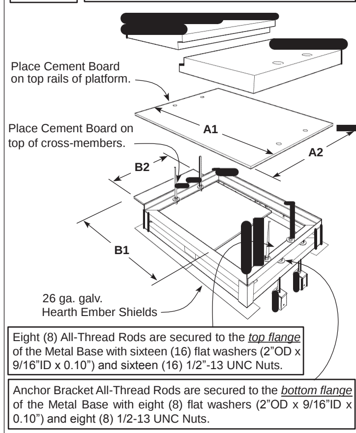
Figure 17 Metal Base Assembly
