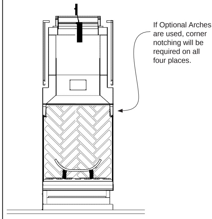
Figure 30 Sectioned Side View
