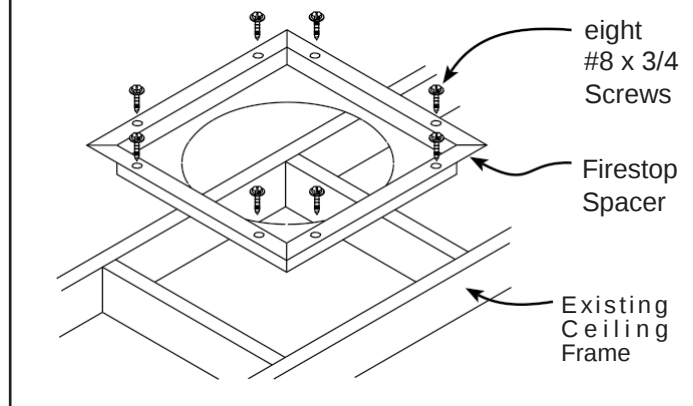
Figure 28 Firestop Spacer with Attic Space Above Ceiling
