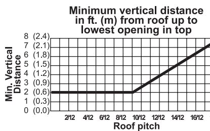
Venting Arrangements - Vertical Terminations with Co-linear Flex System for both Residential & Manufactured Homes into Masonry Fireplaces
