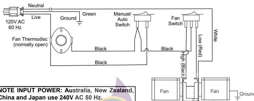
Blower/Fan Wiring Diagram
