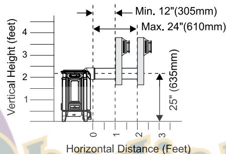
Venting Arrangements - Horizontal Terminations using Dura-Vent venting system and/or Riser Vent Termination
