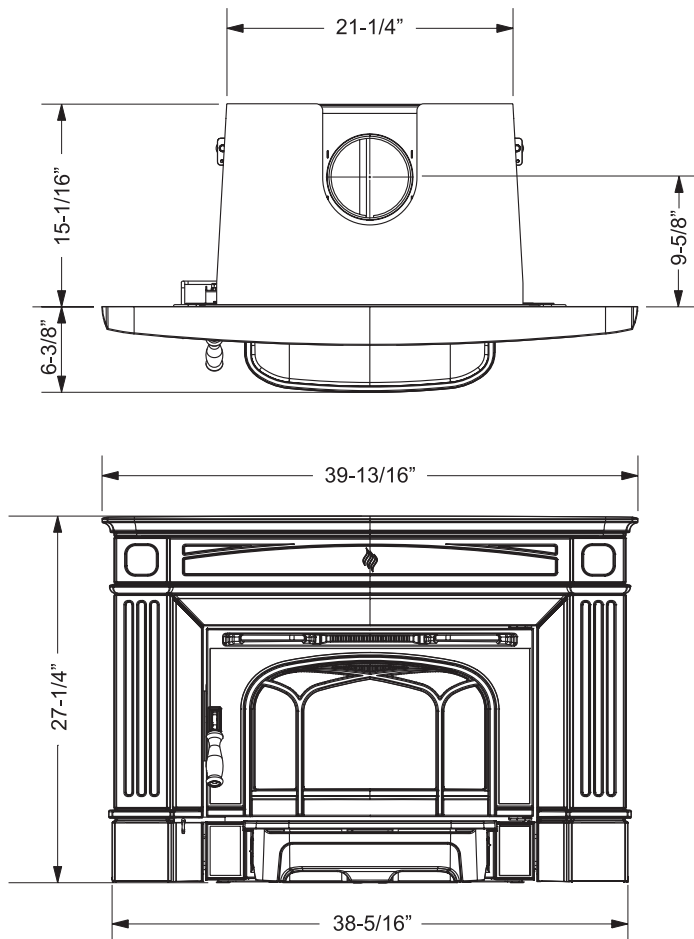
Unit Dimensions with Standard Flue Adaptor
