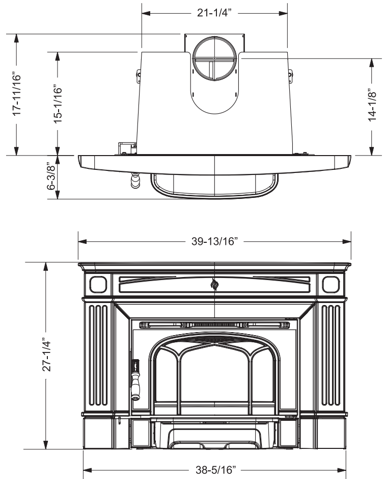
Unit Dimensions with Offset Flue Adaptor
