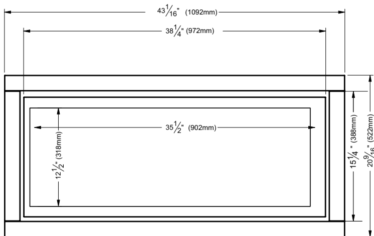
Inner/Outer Faceplate
