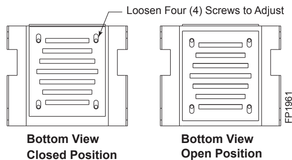
Figure 10 - Baffle Assembly and Adjustment
