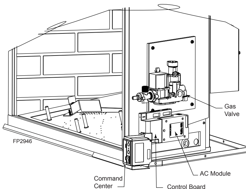
Figure 1 - ICFDV Series Fireplace Insert Controls
