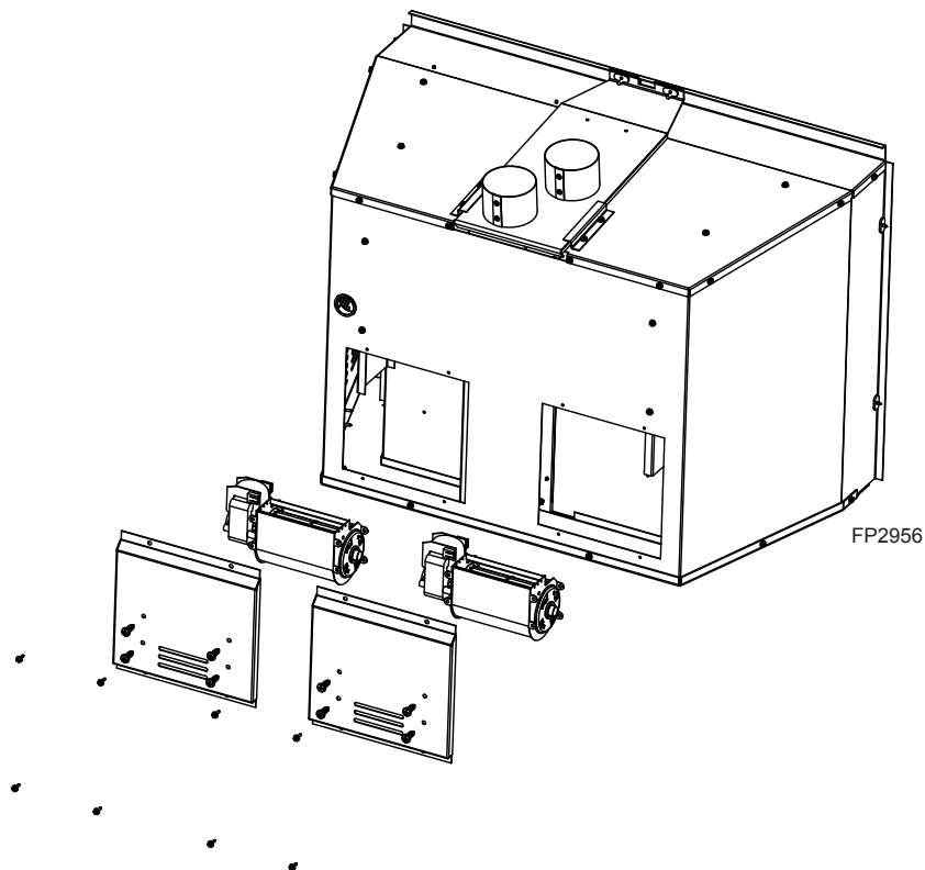
Figure 45 - Blower Removal and Assembly
