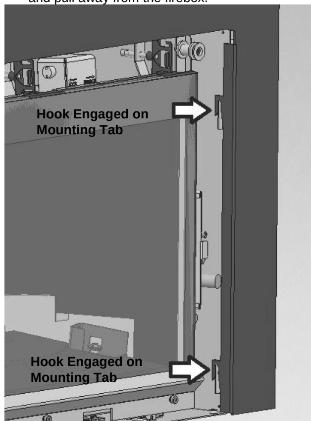
Figure 28 - Surround Mounting Tab Detail
