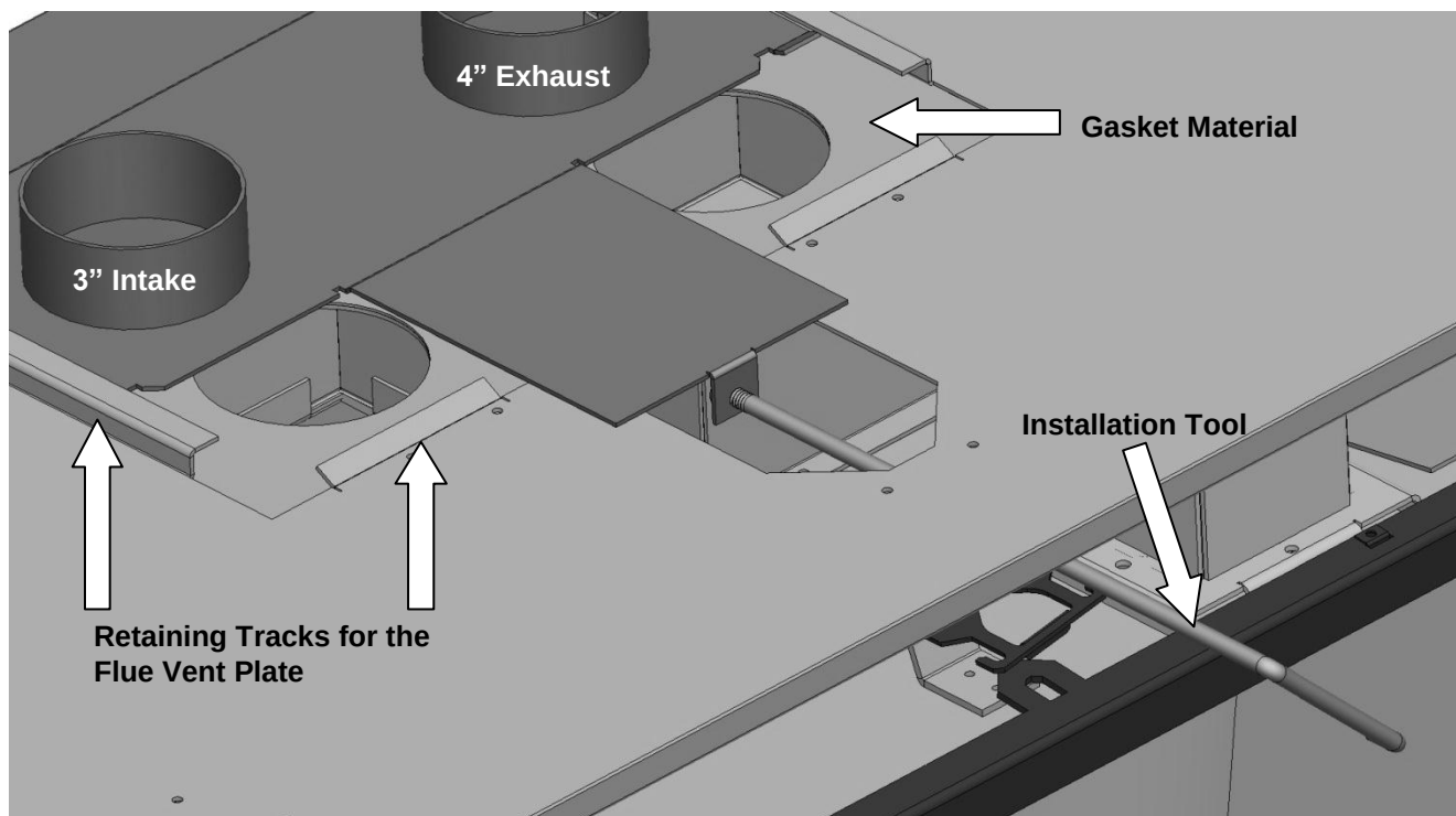
Figure 19 – Flue Plate & Installation Tool Detail
