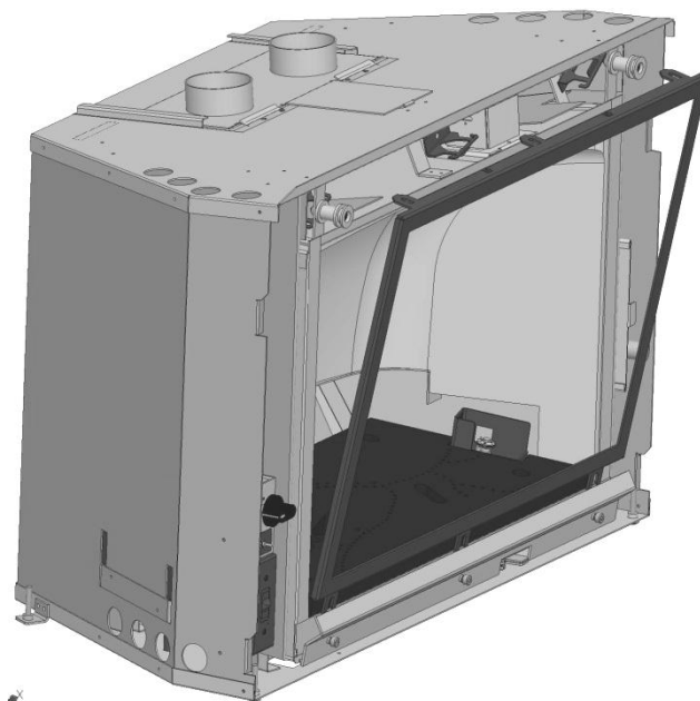
Figure 15 – Tilt and Lift Glass Frame
