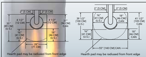
Floor protection for stoves only in the locked position
