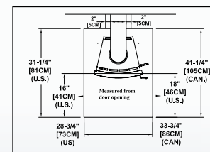
Floor protection
