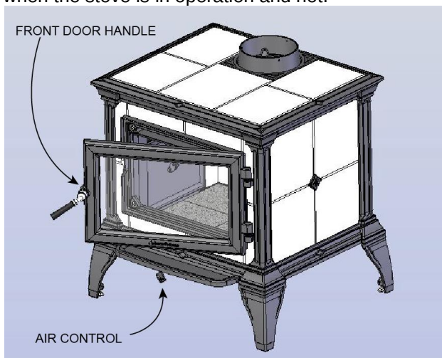
Figure 11 - Controls & Features
