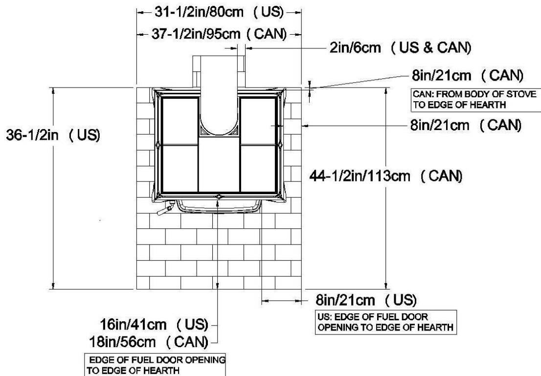
Figure 2 – Hearth Dimensions
