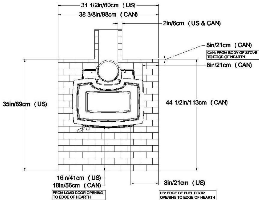
Hearth Dimensions
