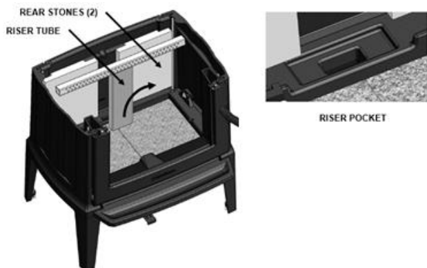
Figure 19 - Removing Riser and Rear Stones
