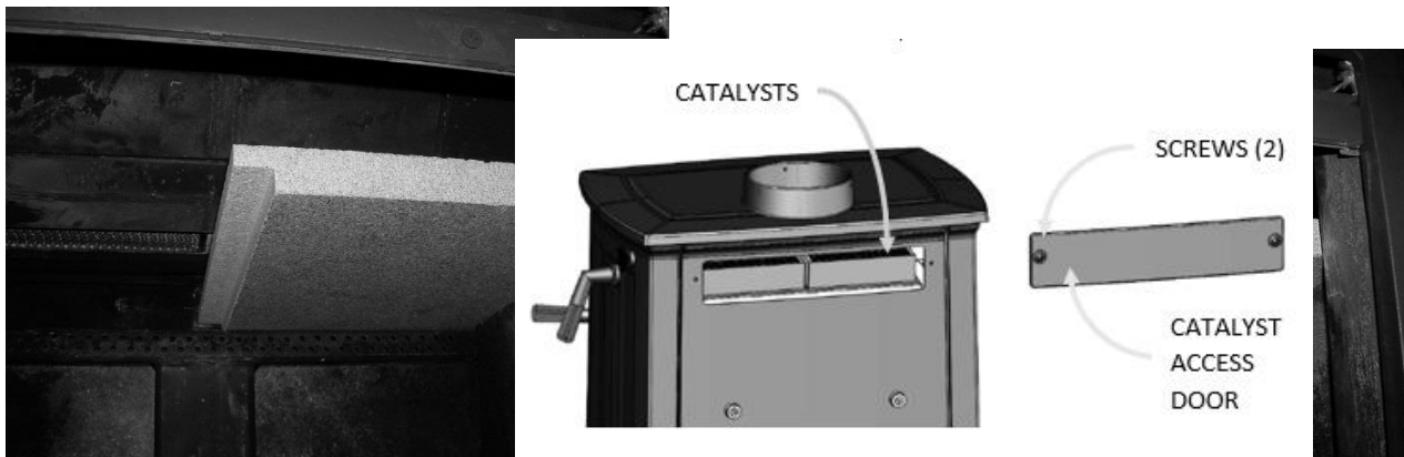
Figure 18 (cont.) - Removing/Replacing Catalyst Access Door
