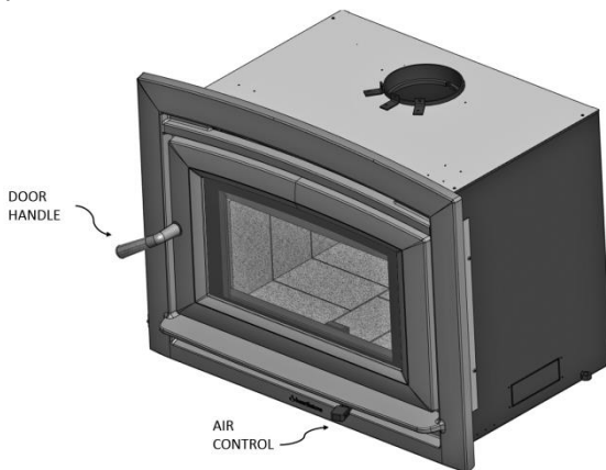
Figure 21 - Controls & Features
