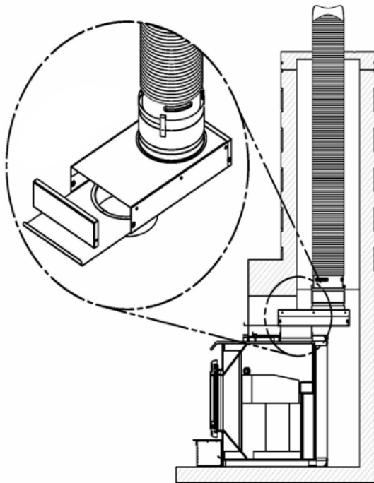
Figure 16 – Offset Adaptor
