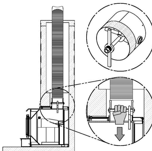
Figure 15 – Liner Fastening System
