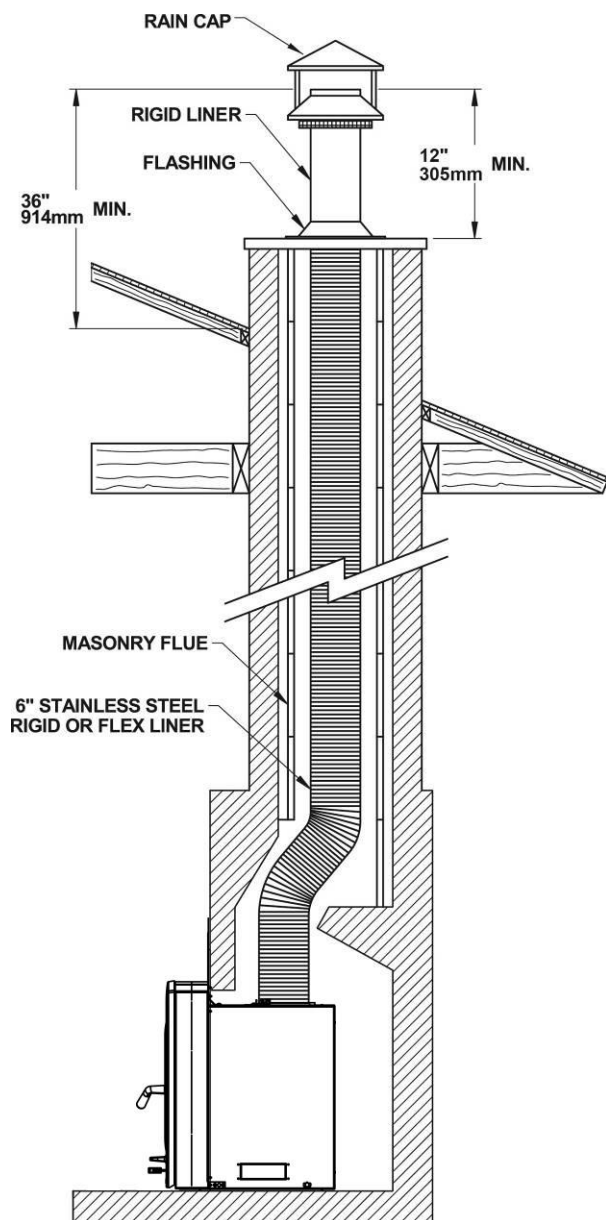
Figure 13 – Liner Installation
