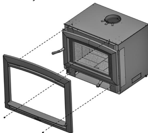
Figure 29 – Remove Front Casting
