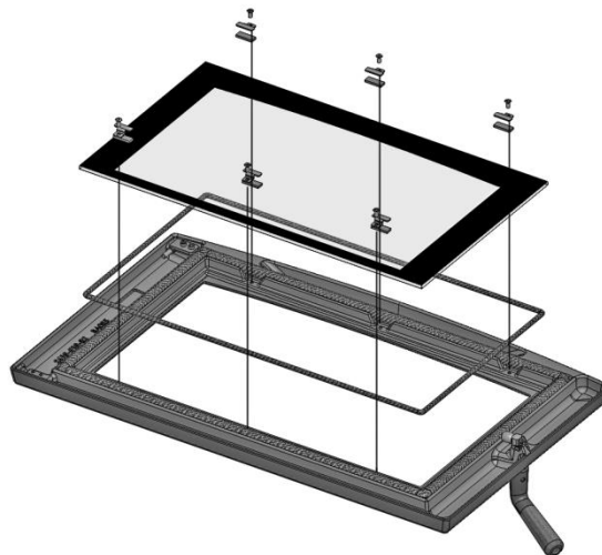
Figure 28 – Glass Assembly
