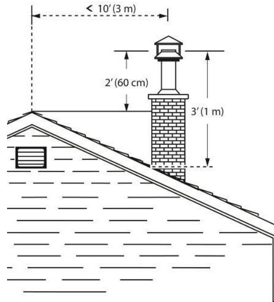
Figure 17 – Min. Chimney Height 1
