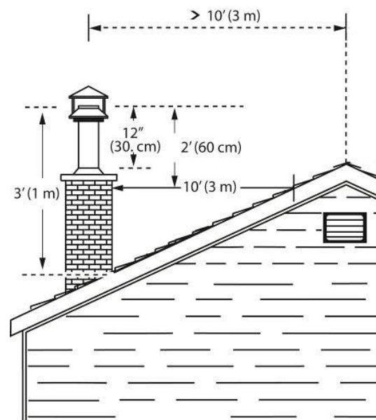
Figure 18 – Min. Chimney Height 2
