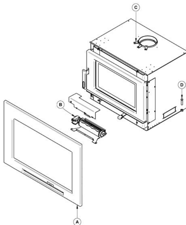
Figure 39 – Insert Removal
