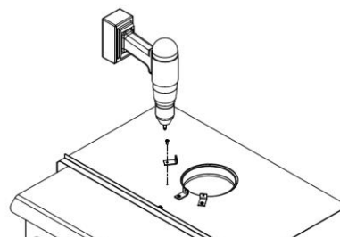
Figure 14 – Liner Connection
