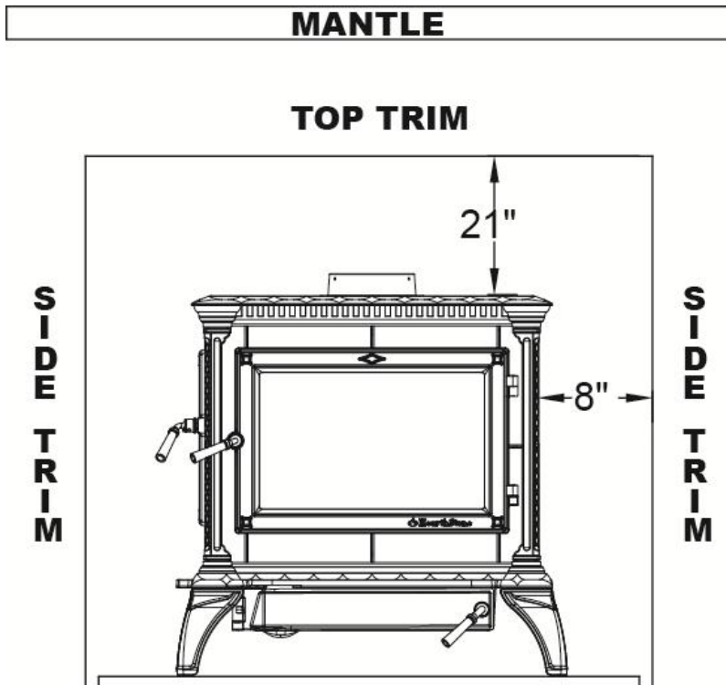
Figure 8 – Mantle Clearances (Front View)
