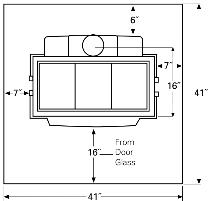
Minimum Hearthpad Dimensions
