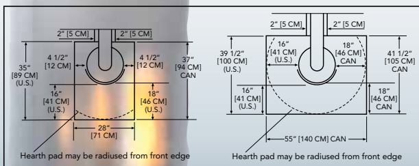
Floor protection for stoves only in the locked position
