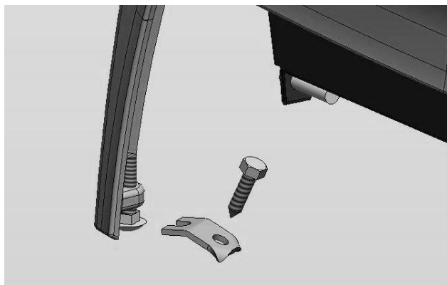
Figure 7 - Lock Down Detail
