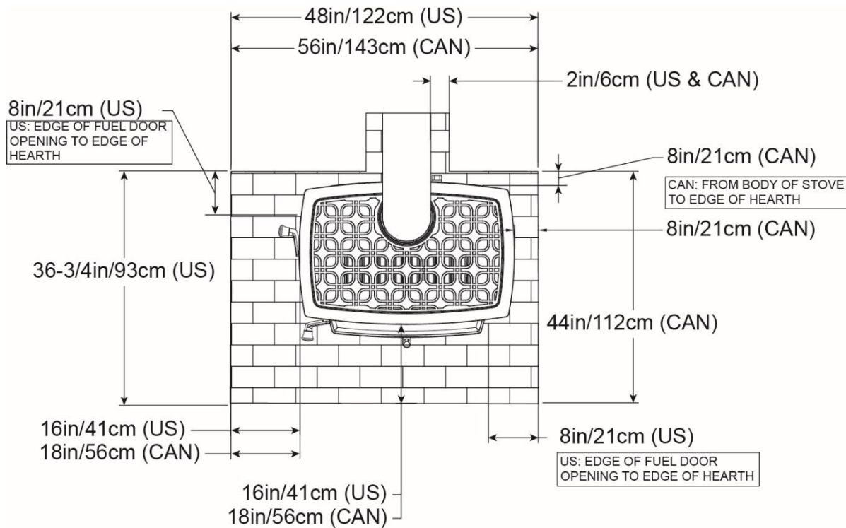
Figure 2 – Hearth Dimensions
