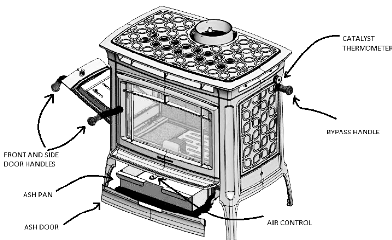
Figure 10 - Controls & Features
