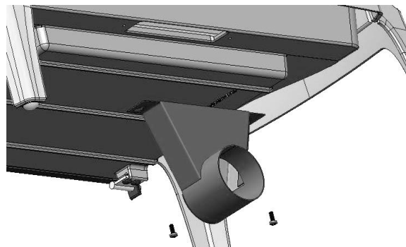
Figure 7 – Outside Air Kit Detail
